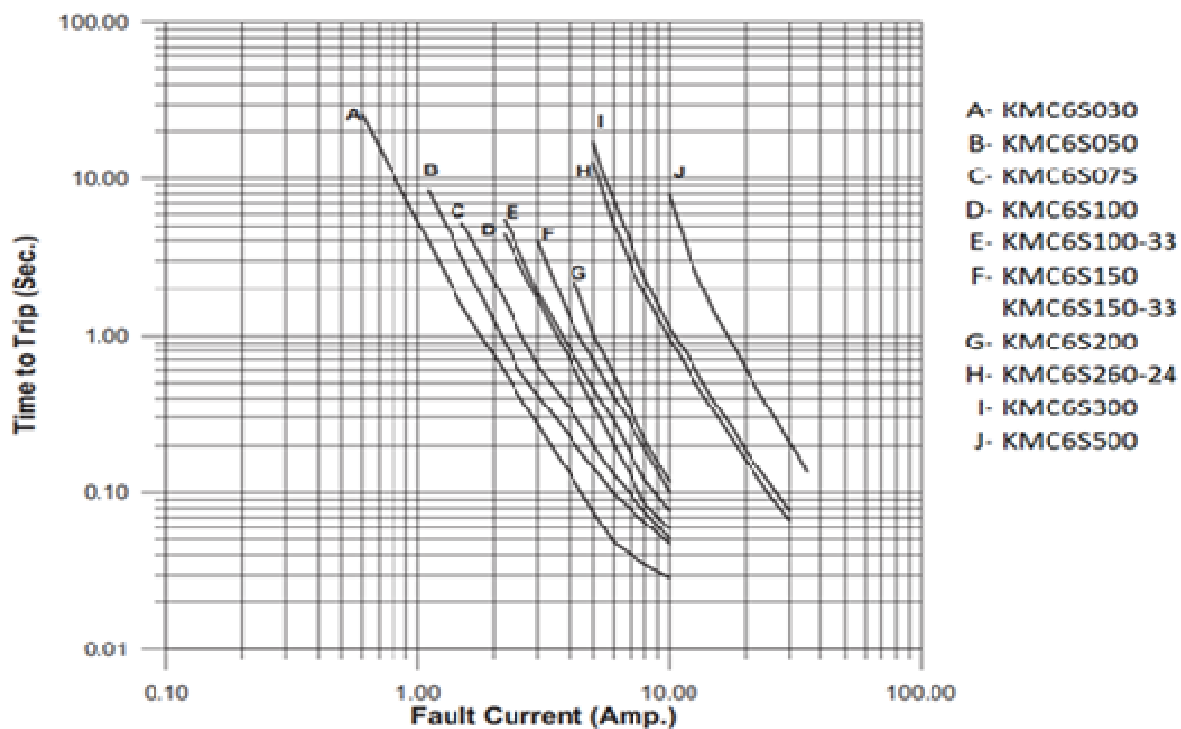
KMC6S: 2018 Series
