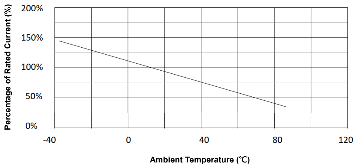
Derating Curve for KMC4S (1210) Series
