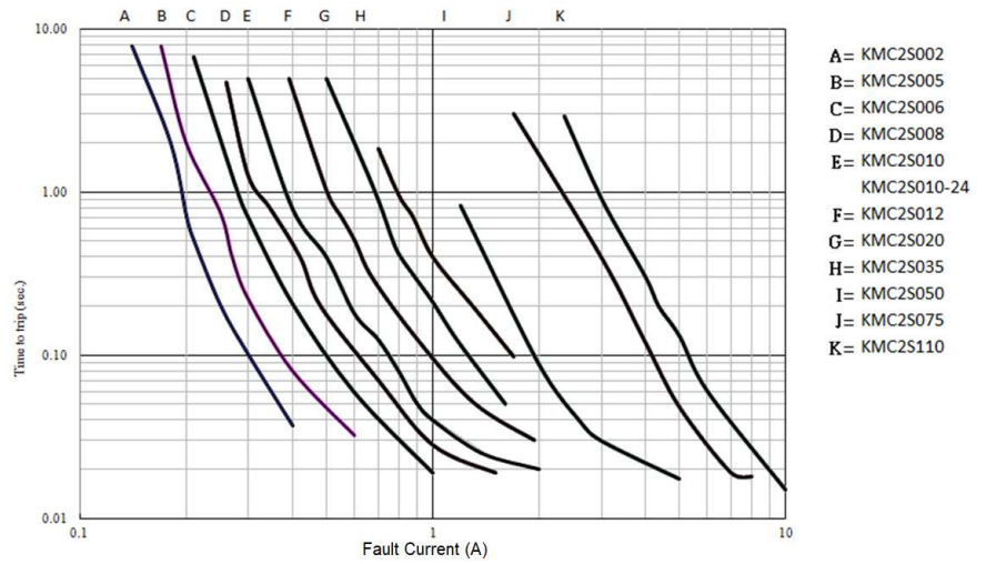
KMC2S: 0805 Series
