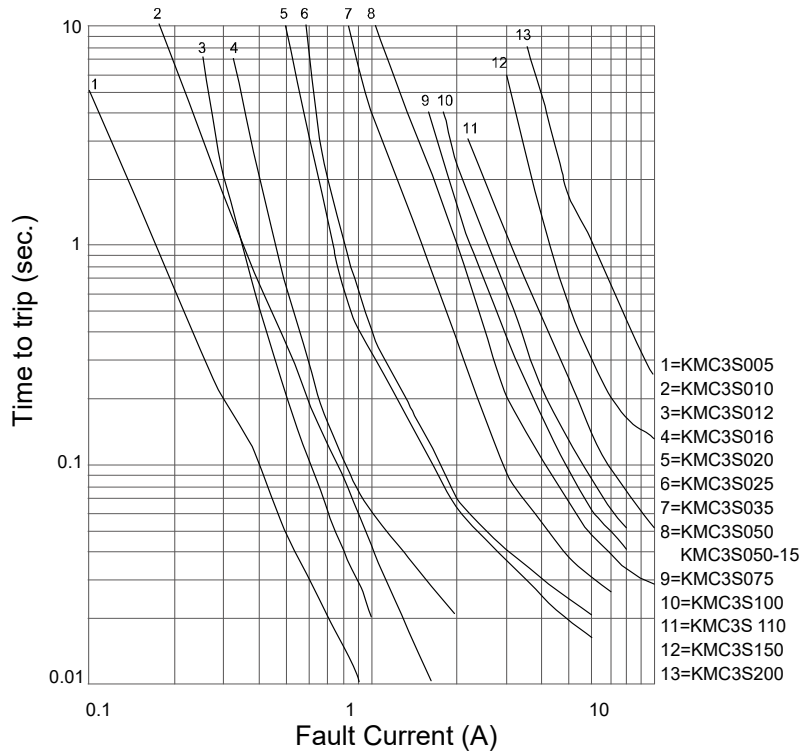
KMC3S: 1206 Series
